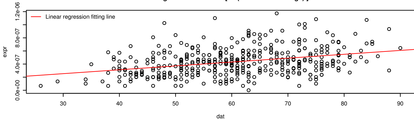
Linear Regression model on [ Im(Mutation rate ~ Age) ]
