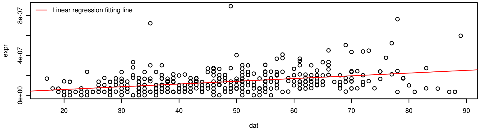
Linear Regression model on [ Im(Mutation rate ~ Age) ]
