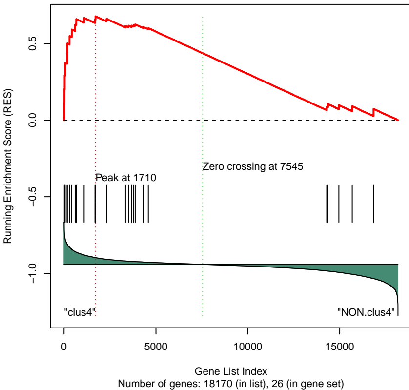
Gene Set 10 : BIOCARTA_INFLAM_PATHWAY
