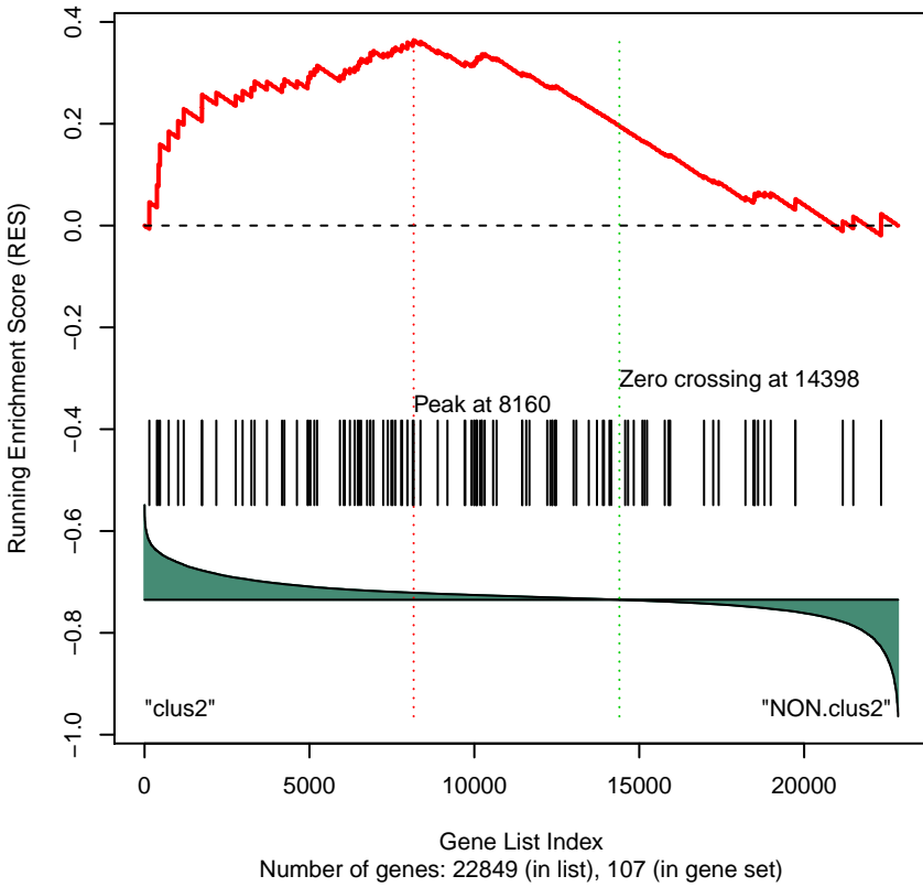
Gene Set 108 : KEGG_OOCYTE_MEIOSIS
