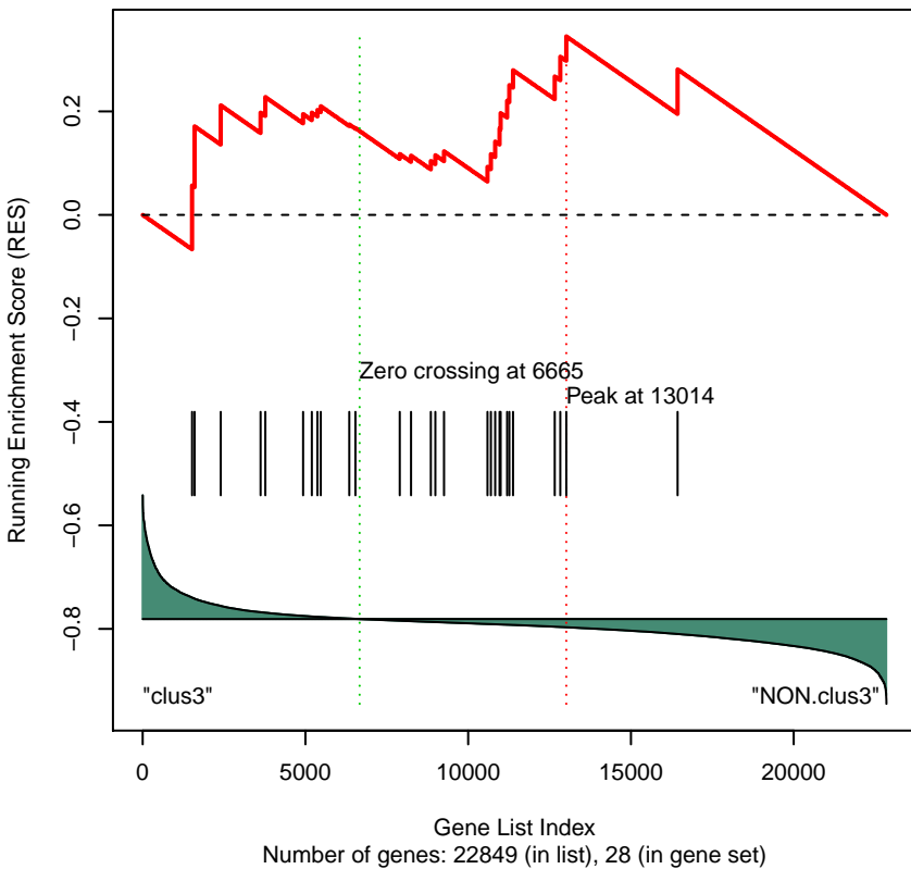
Gene Set 91 : KEGG_RNA_POLYMERASE
