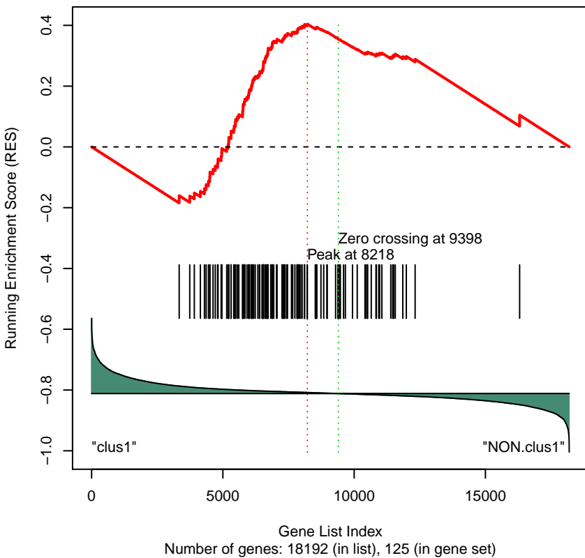
Gene Set 90 : KEGG_SPLICEOSOME
