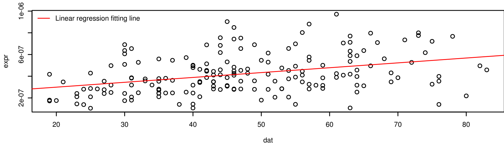
Linear Regression model on [ Im(Mutation rate ~ Age) ]
