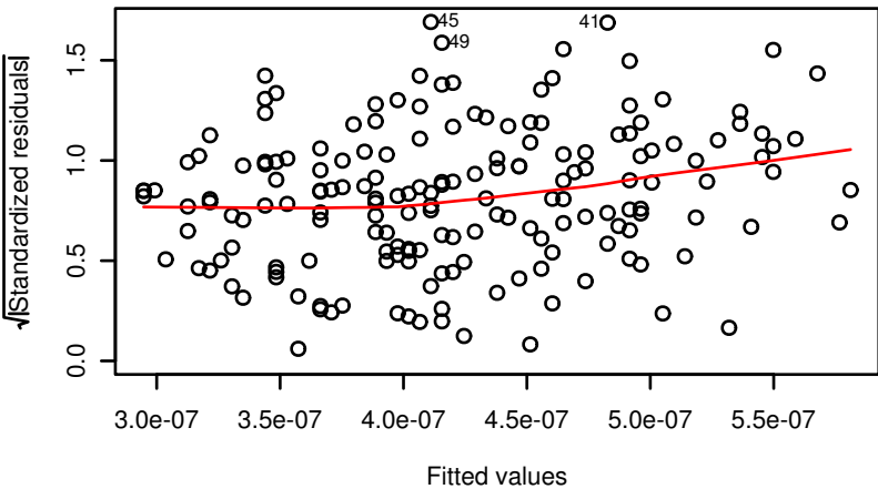
Scale-Location
