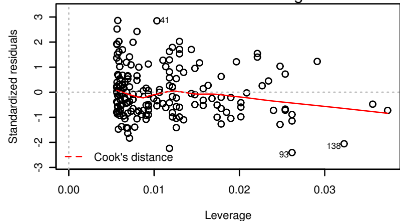
Residuals vs Leverage
