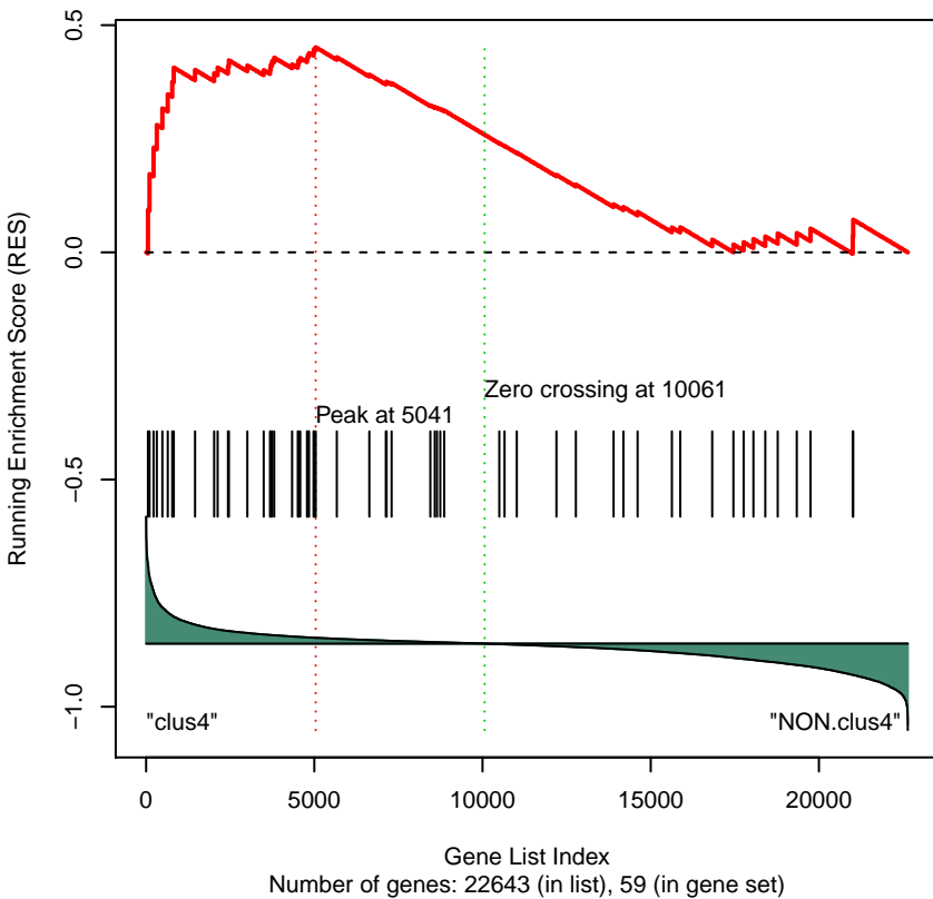
Gene Set 46 : KEGG_GLYCOLYSIS_GLUCONEOGENESIS
