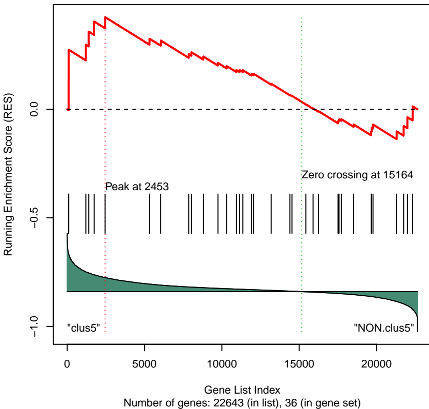
Gene Set 41 : BIOCARTA_PAR1_PATHWAY
