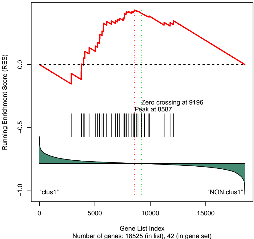
Gene Set 94 : KEGG_PROTEASOME
