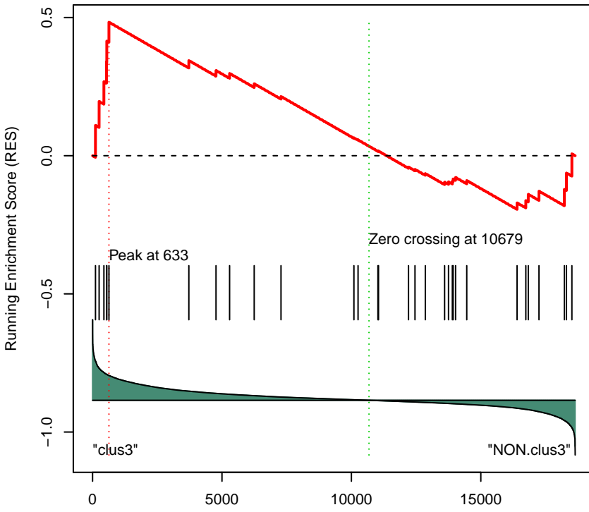
Gene Set 78 : KEGG_BUTANOATE_METABOLISM
