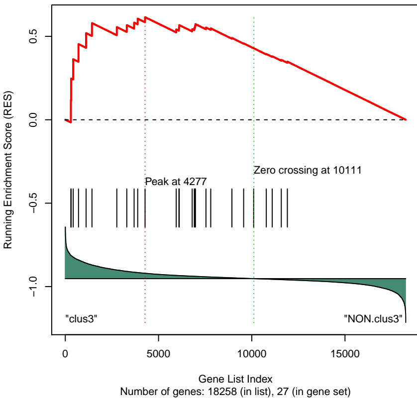
Gene Set 99 : KEGG_HOMOLOGOUS_RECOMBINATION
