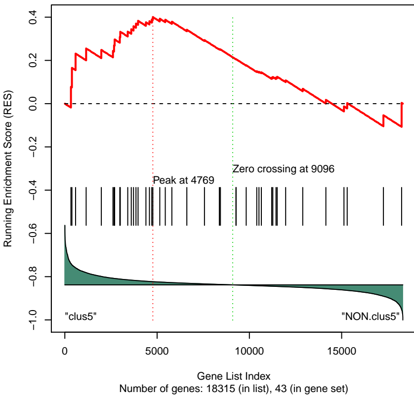
Gene Set 64 : KEGG_GLUTATHIONE_METABOLISM
