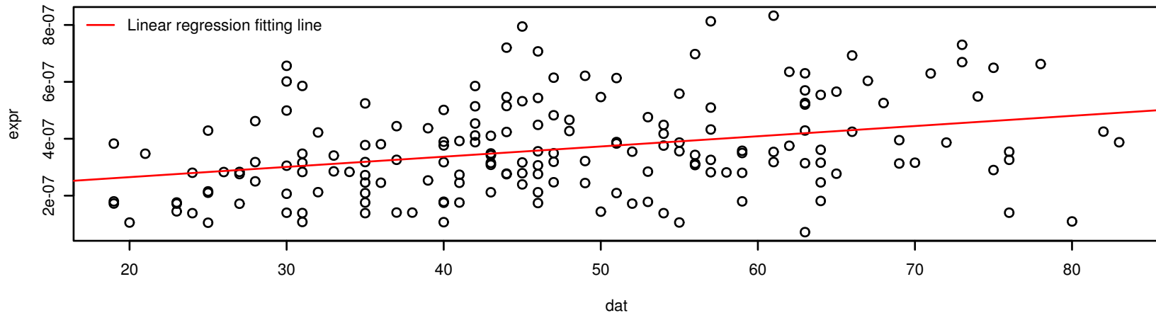
Linear Regression model on [ Im(Mutation rate ~ Age) ]
