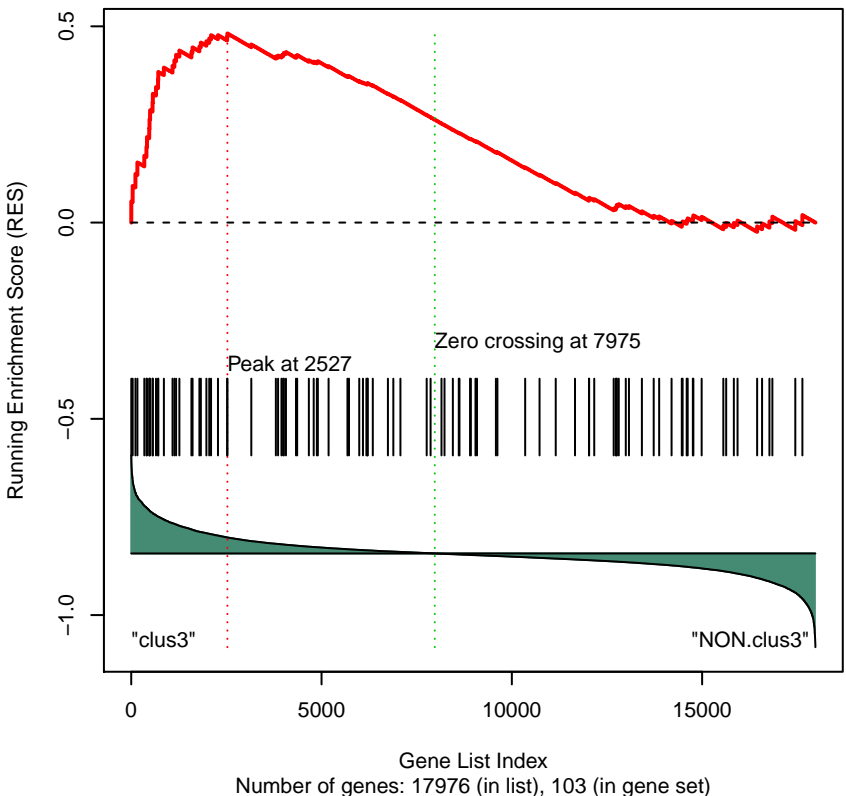
Gene Set 111 : KEGG_VASCULAR_SMOOTH_MUSCLE_CONTRACTIC
