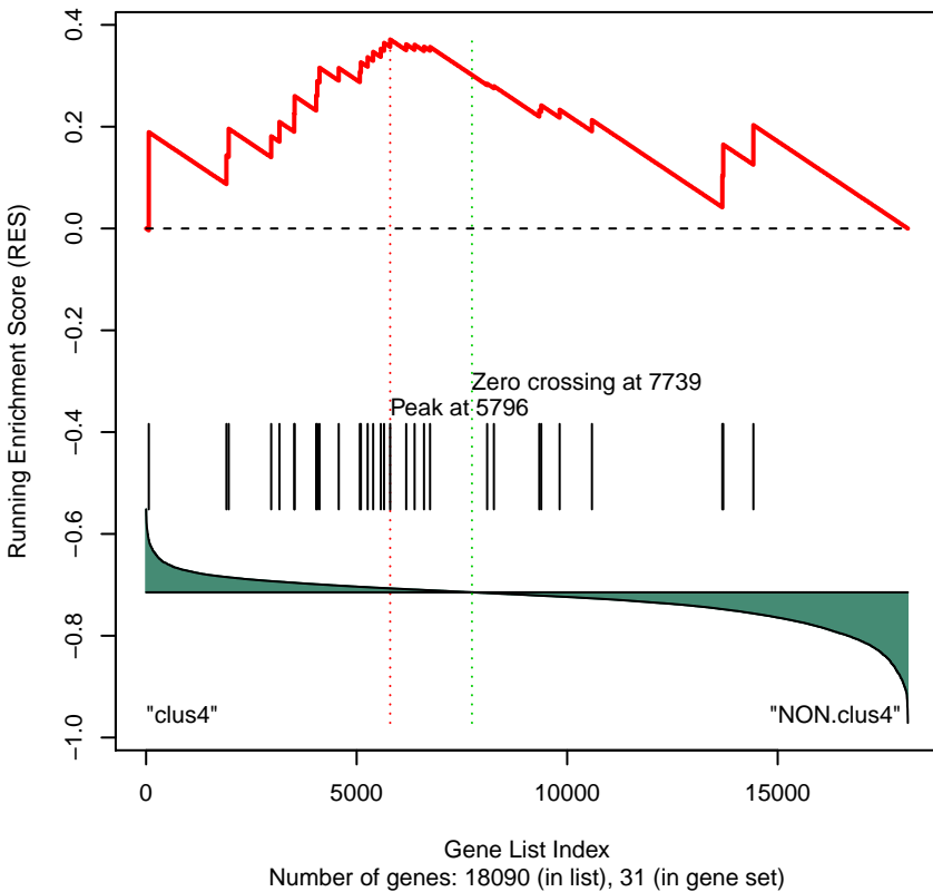
Gene Set 79 : KEGG_PROANOATE_METABOLISM
