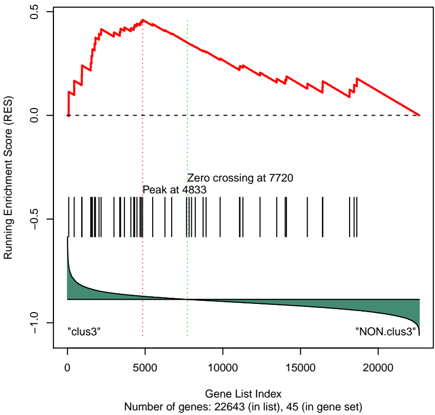
Gene Set 66 : KEGG_GLUTATHIONE_METABOLISM
