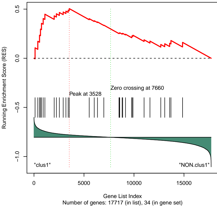
Gene Set 272 : PID_ATM_PATHWAY
