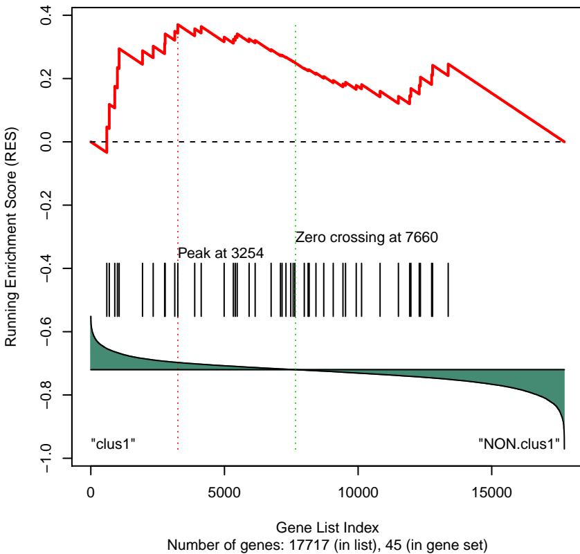
Gene Set 264 : PID_ILK_PATHWAY
