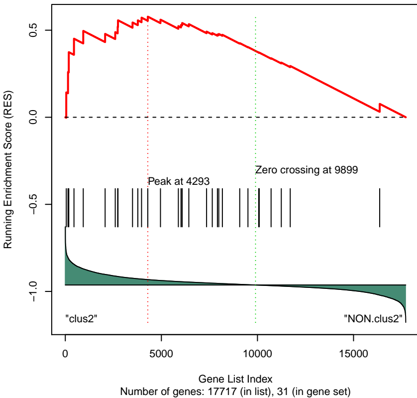
Gene Set 219 : ST_WNT_BETA_CATENIN_PATHWAY
