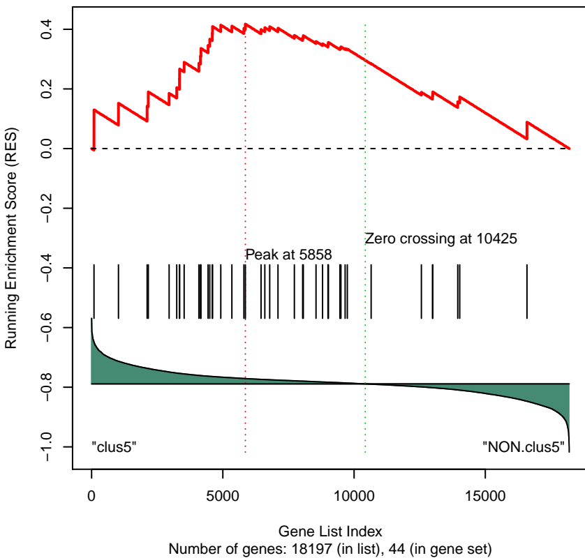
Gene Set 15 : KEGG_LYSINE_DEGRADATION
