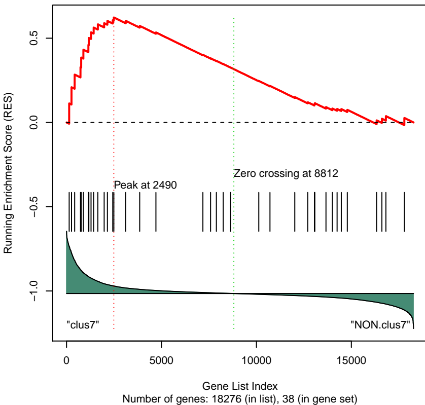
Gene Set 18 : KEGG_TRYPTOPHAN_METABOLISM
