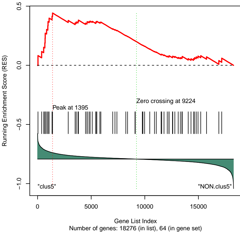
Gene Set 373 : PID_RB_1PATHWAY
