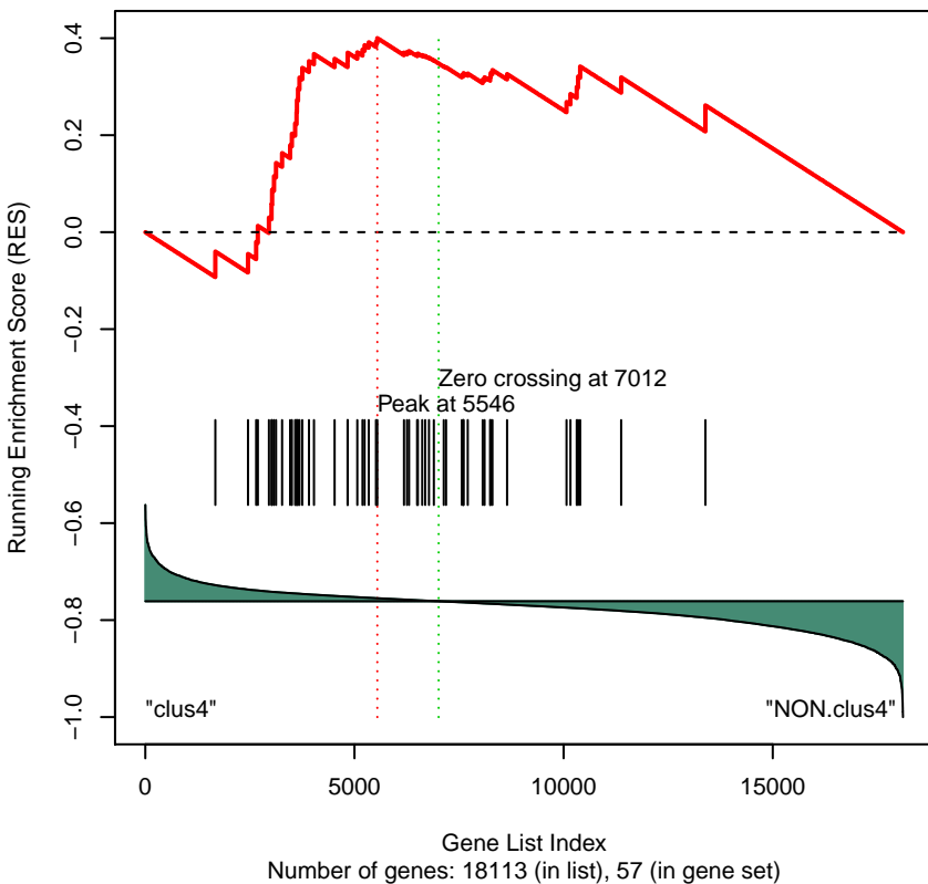
Gene Set 403 : REACTOME_ER_PHAGOSOME_PATHWAY
