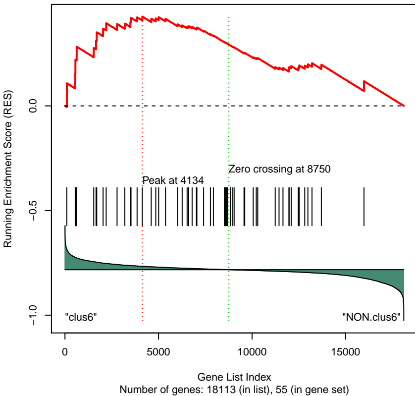
Gene Set 380 : PID_TGFBRPATHWAY
