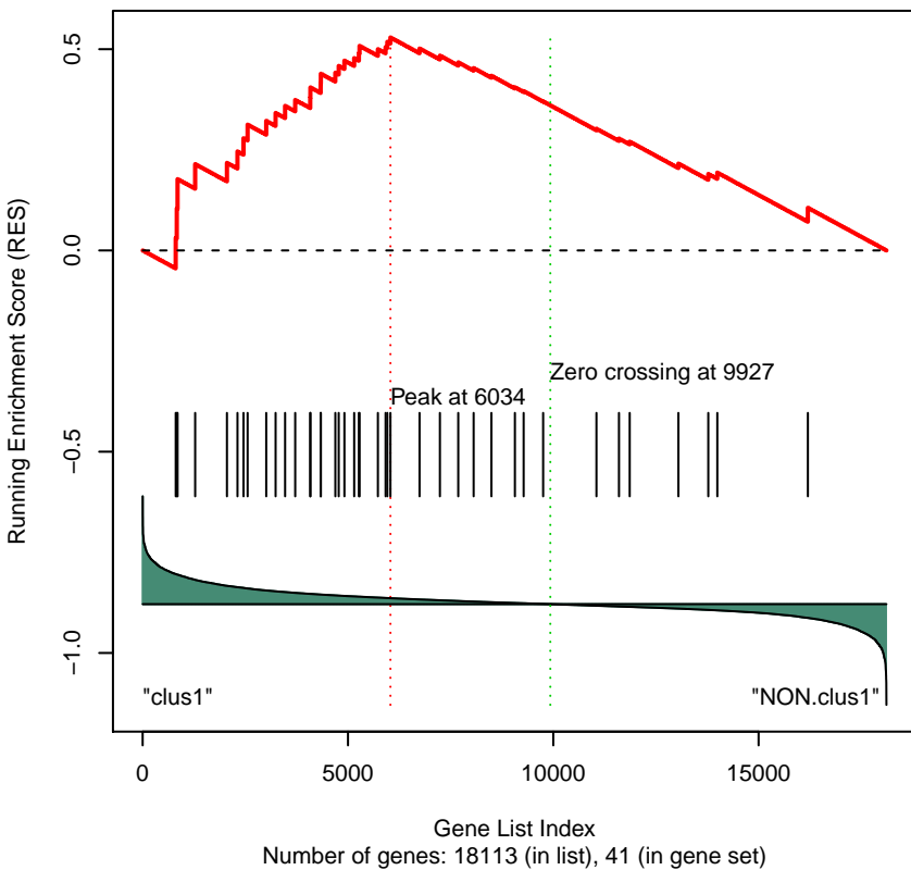
Gene Set 250 : PID_ER_NONGENOMIC_PATHWAY
