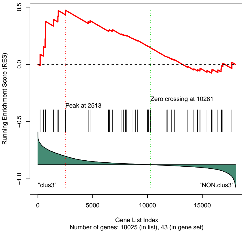
Gene Set 44 : KEGG_ABC_TRANSPORTERS
