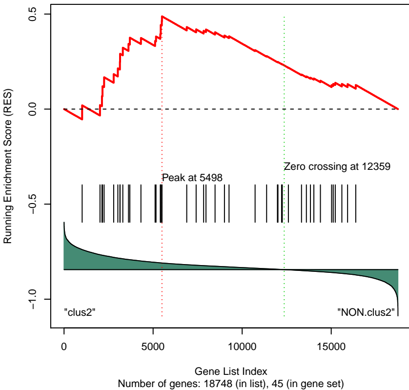
Gene Set 302 : PID_PLK1_PATHWAY
