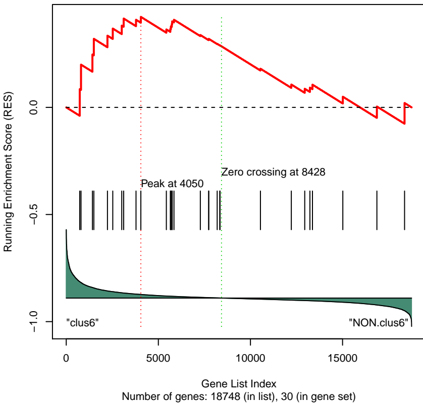
Gene Set 339 : PID_RETINOIC_ACID_PATHWAY
