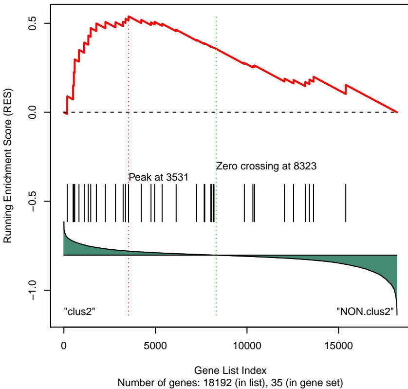
Gene Set 328 : PID_HIVNEFPATHWAY
