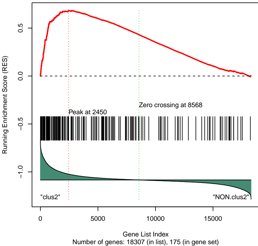
Gene Set 57 : KEGG_CALCIUM_SIGNALING_PATHWAY
