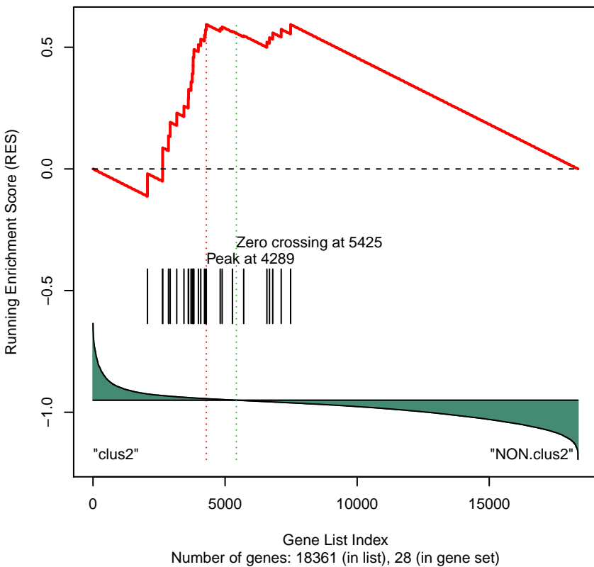
Gene Set 182 : BIOCARTA_PROTEASOME_PATHWAY
