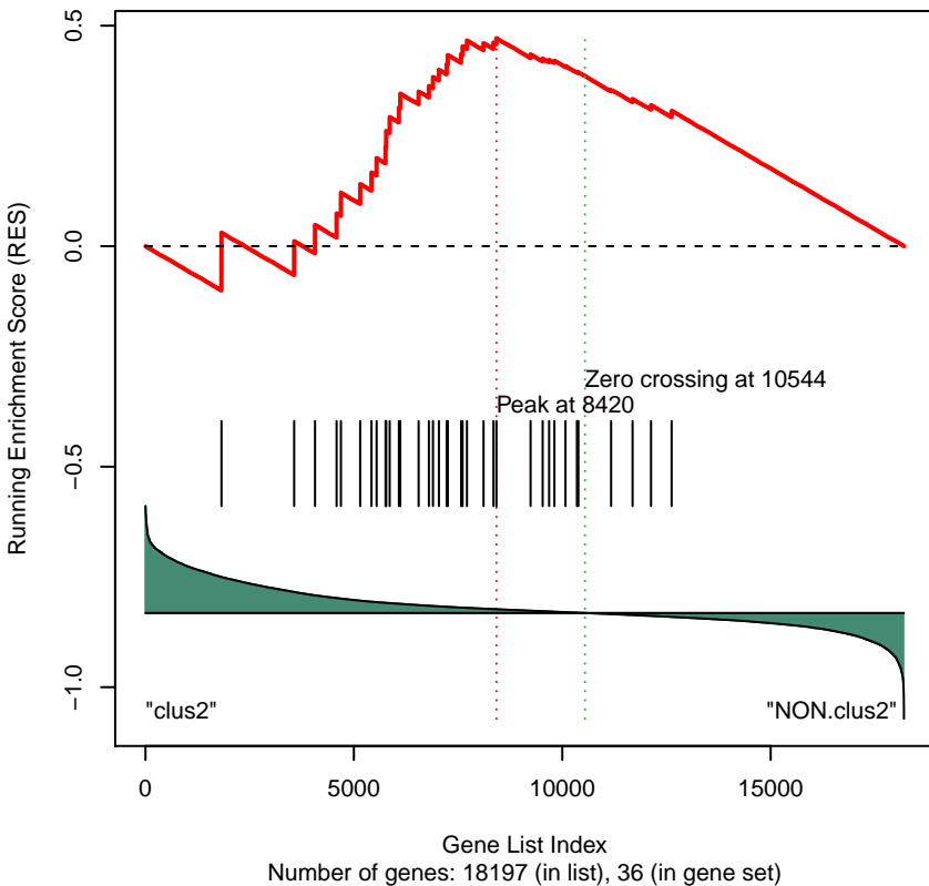
Gene Set 50 : KEGG_DNA_REPLICATION
