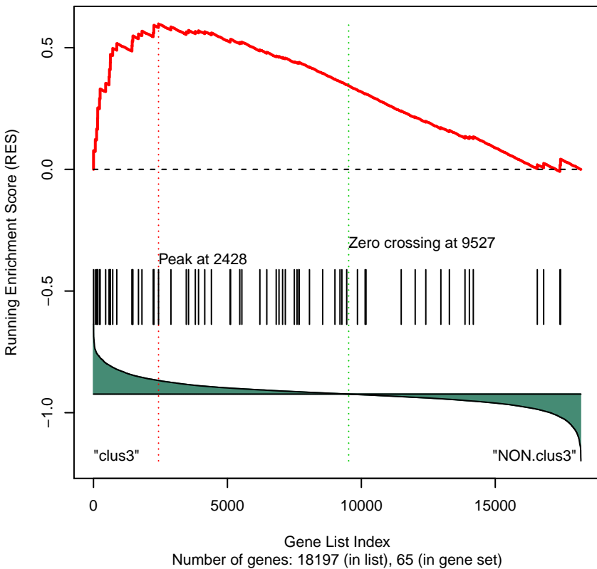
Gene Set 53 : KEGG_PPAR_SIGNALING_PATHWAY
