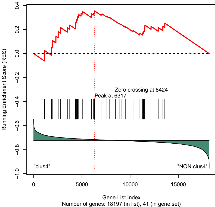
Gene Set 41 : KEGG_AMINOACYL_TRNA_BIOSYNTHESIS
