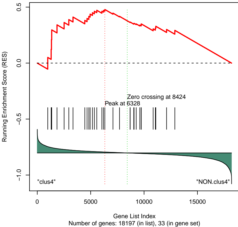
Gene Set 54 : KEGG_BASE_EXCISION_REPAIR
