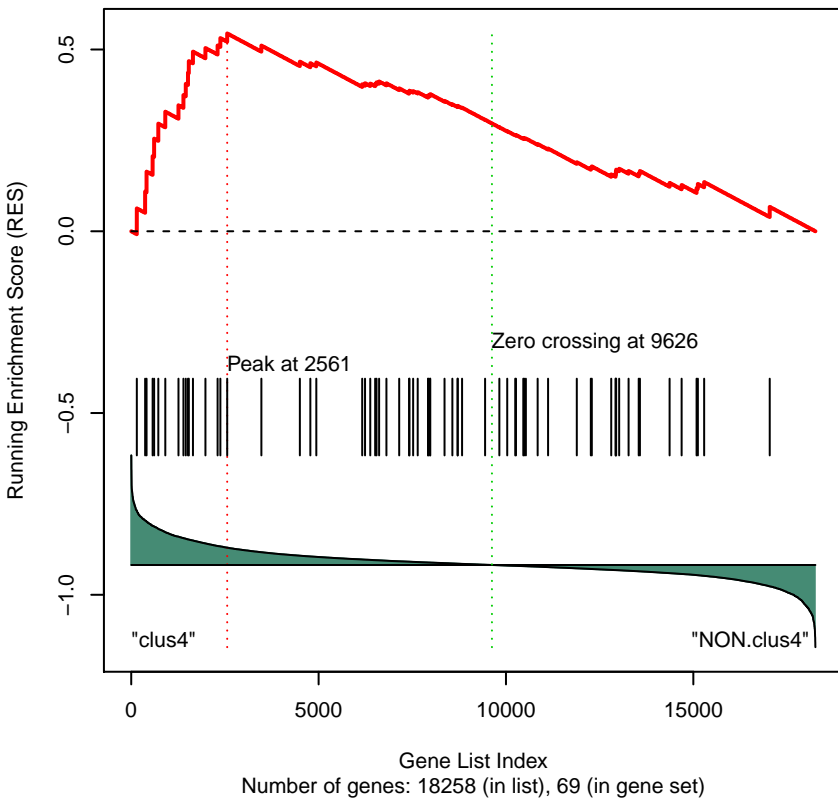
Gene Set 249 : PID_E2F_PATHWAY
