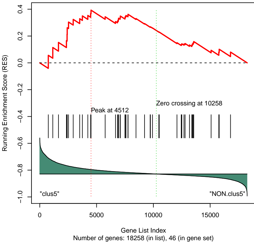
Gene Set 77 : KEGG_NOTCH_SIGNALING_PATHWAY
