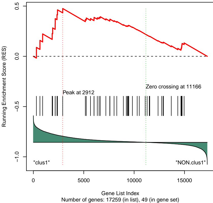
Gene Set 69 : KEGG_MTOR_SIGNALING_PATHWAY
