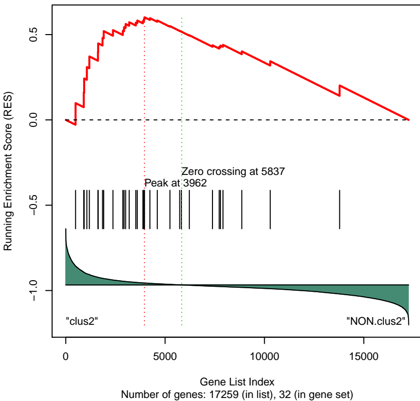
Gene Set 360 : PID_MAPKTRKPATHWAY
