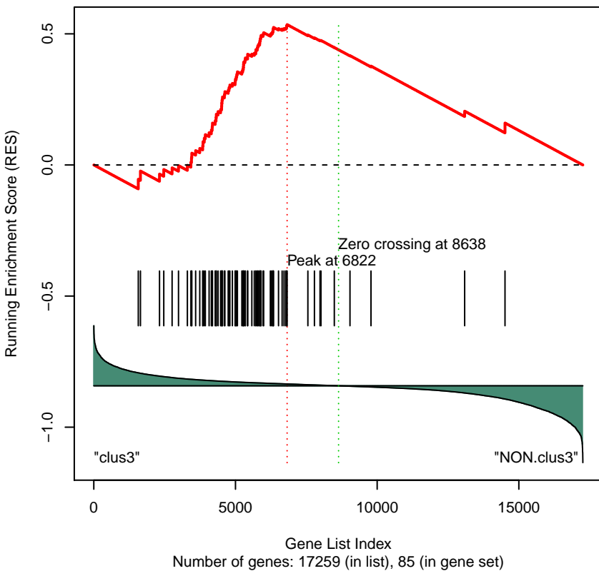
Gene Set 43 : KEGG_RIBOSOME
