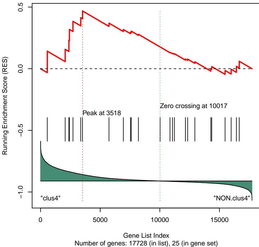
Gene Set 6 : KEGG_GALACTOSE_METABOLISM
