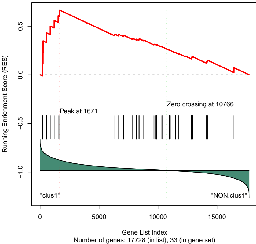
Gene Set 300 : PID_IL2_PI3KPATHWAY
