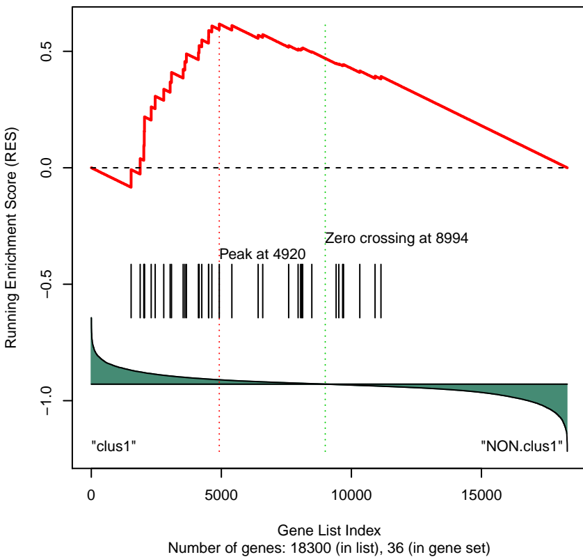
Gene Set 49 : KEGG_DNA_REPLICATION
