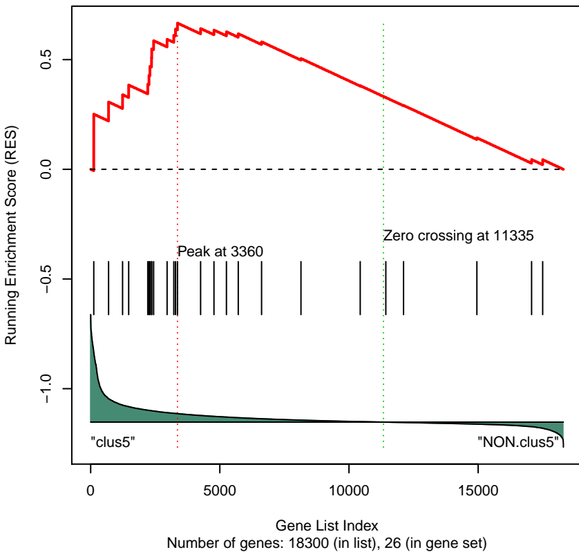
Gene Set 32 : KEGG_LINOLEIC_ACID_METABOLISM
