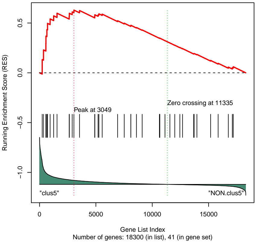
Gene Set 17 : KEGG_TYROSINE_METABOLISM
