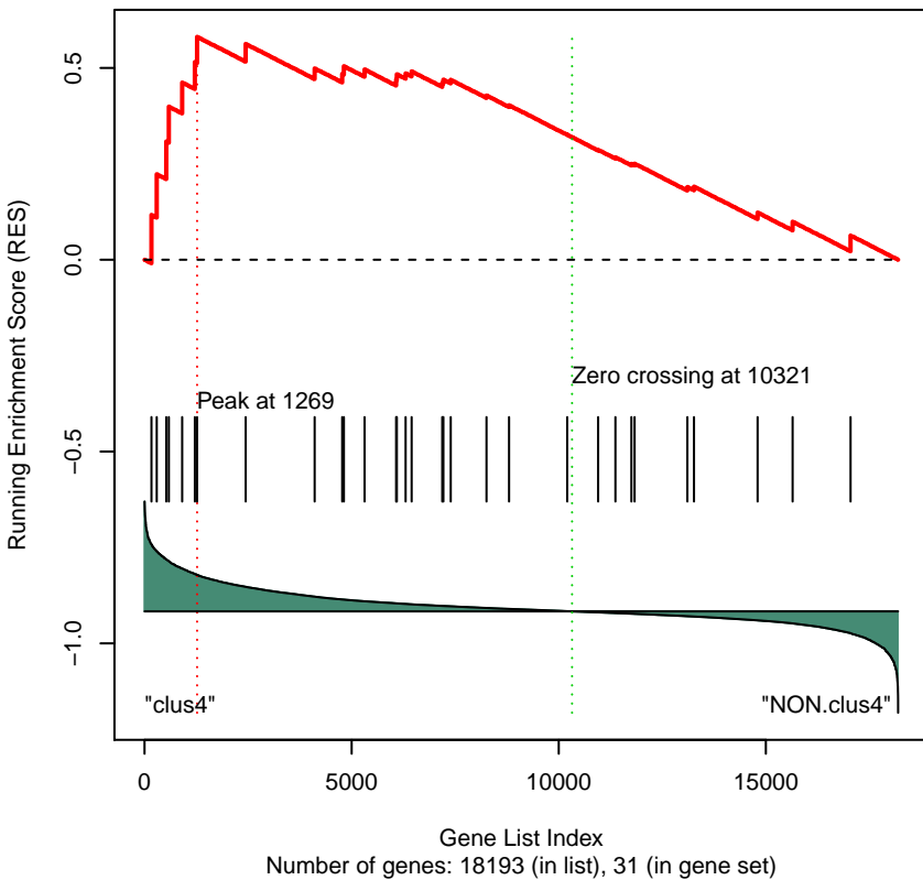
Gene Set 218 : ST_WNT_BETA_CATENIN_PATHWAY
