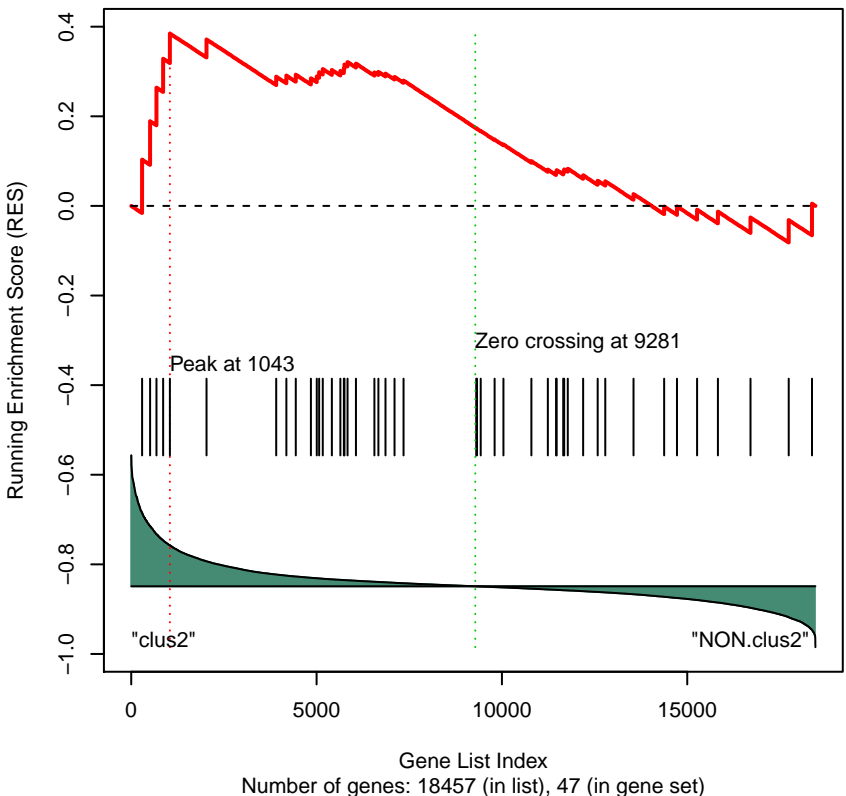
Gene Set 281 : PID_LKB1_PATHWAY
