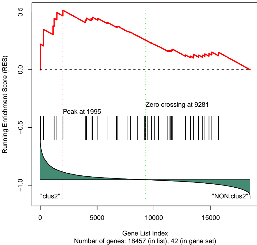
Gene Set 159 : BIOCARTA_BIOPEPTIDES_PATHWAY
