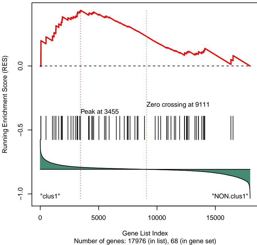
Gene Set 100 : KEGG_LONG_TERM_POTENTIATION
